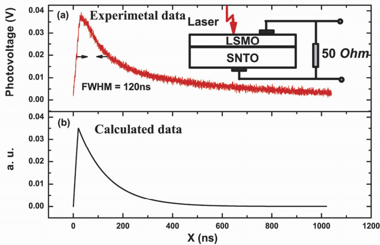
Fig. 6. (a) Experimental evolution of photovoltage in the LSMO1/SNTO heterostructure connected with 50 \Omega resistance. The inset presents the illustration of heterostructure for voltaic measurement. (b) The calculated evolution of photovoltage.
