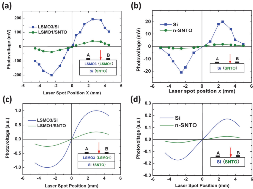
Fig. 7. The experimental (a) and theoretical (c) LPVs of the LSMO side in the LSMO1/SNT0 denoted by the green curve and LSMO3/Si denoted by the blue curve; the experimental (b) and theoretical (d) LPVs of SNT0 denoted by the green curve and Si denoted by the blue curve. The photovoltage denotes the peak value of LPV between the indium electrodes A ( x = -3 mm) and B ( x = 3 mm). The inset shows the schematic setup for LPV measurement.
