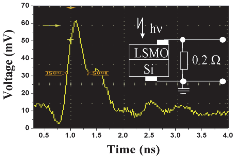
Fig. 2. Variation of the photovoltage with time under the same condition as in Fig. 1, but with a 0.2\ \Omega resistance connected in parallel across the heterostructure. Inset displays a schematic circuit of the sample measurement.
