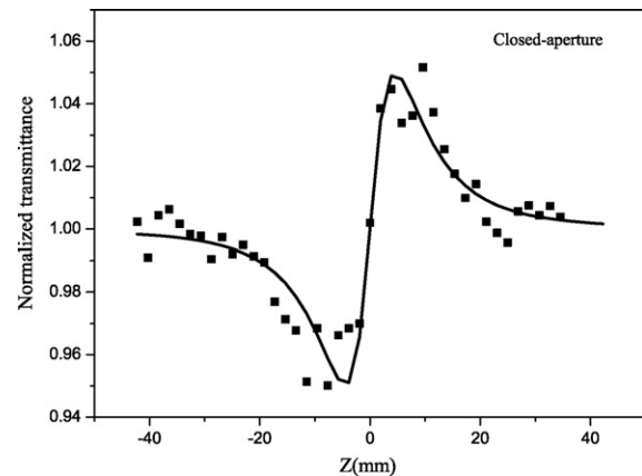
Fig. 5. z -Scan normalized transmittance with closed-aperture of Au/ZnO nanoparticle arrays. The solid curve is the theoretical fit to the data.
