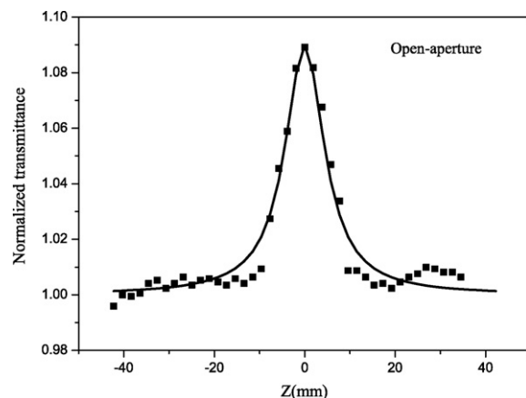
Fig. 6. z -Scan normalized transmittance with open-aperture of Au/ZnO nanoparticle arrays. The solid curve is the theoretical fit to the data.
