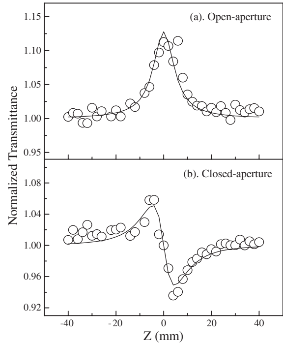
Figure 4. Z-scan results of N3 with open (a) and closed (b) aperture. The solid lines indicate the theoretical fit.
