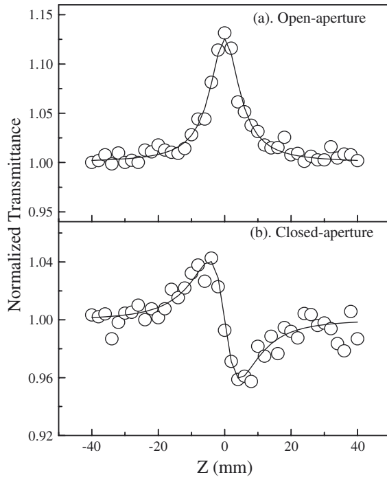
Figure 3. Z-scan results of N1 with open (a) and closed (b) aperture. The solid lines indicate the theoretical fit.
