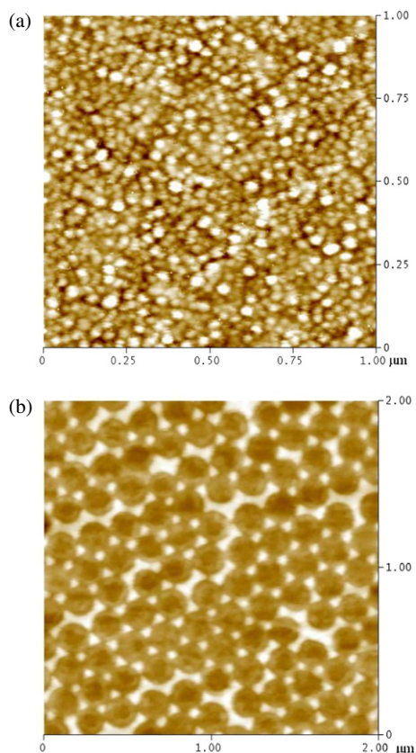
Figure 1. AFM images of the ultra-thin gold film and nanoparticle arrays: (a) N1 (film, 12 nm); (b) N3 (array, 14 nm).
